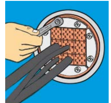
6 Tighten the nuts so that 10-12 mm of the protruding thread is visible.
