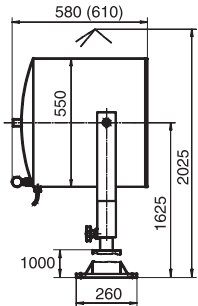
NHS550B Gewicht/ weight: 26.7 kg
