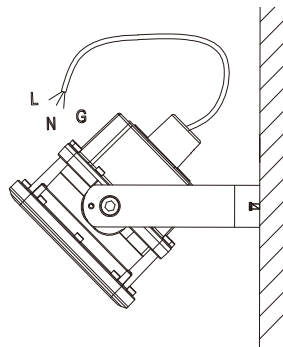
2 - Veggmontering
