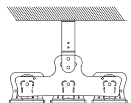
Ceiling installation
