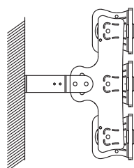
Wall installation
